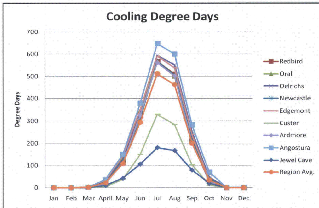
Figure 3-10. Cooling Degree Days for Regional Stations [High Plains Regional Climate Center, 2008; South Dakota State University, 2008].
