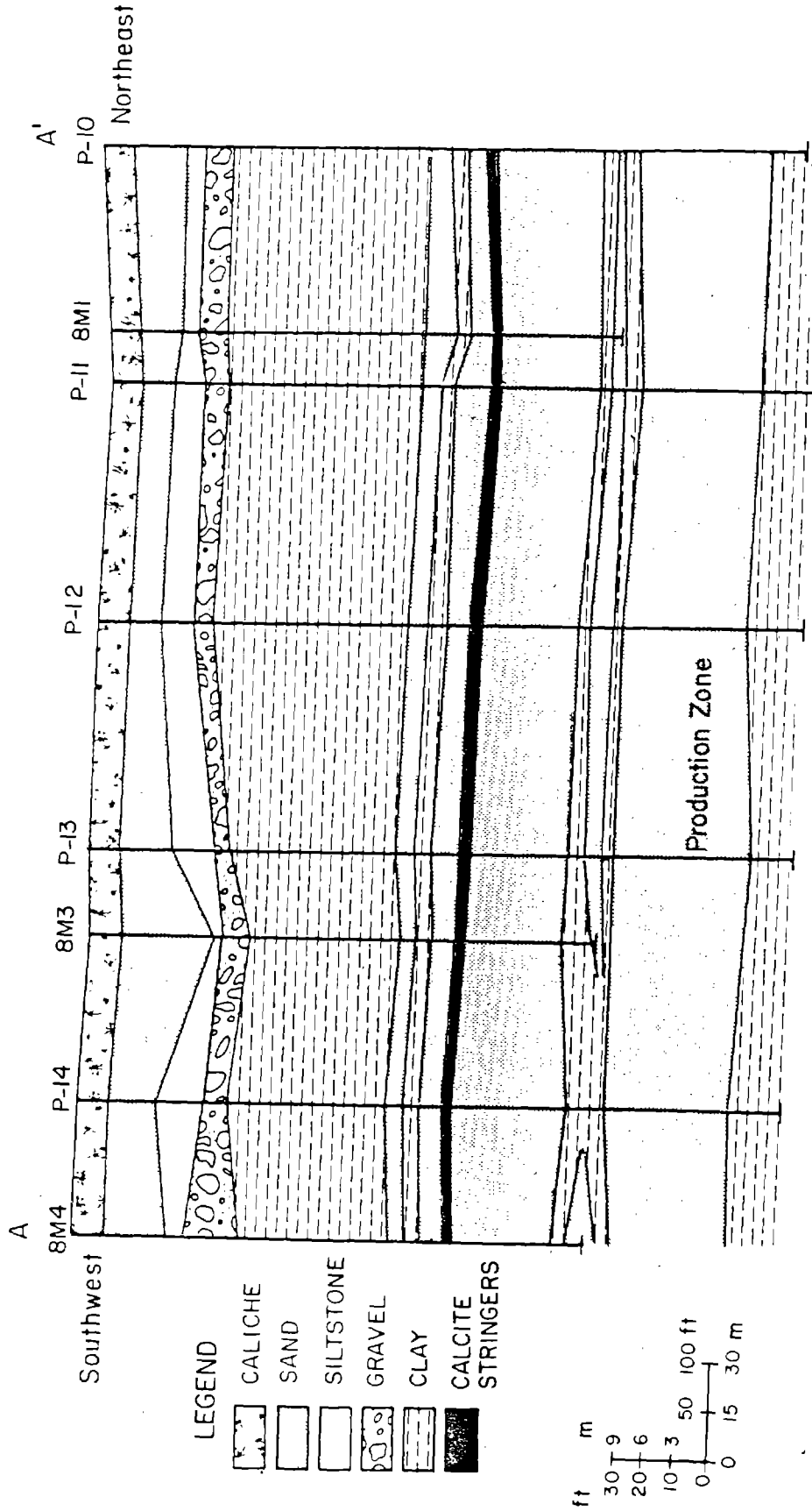
Fig. A.63. Simplified geologic cross section through the Bruni mine site. Source: WMC, 1979a.
