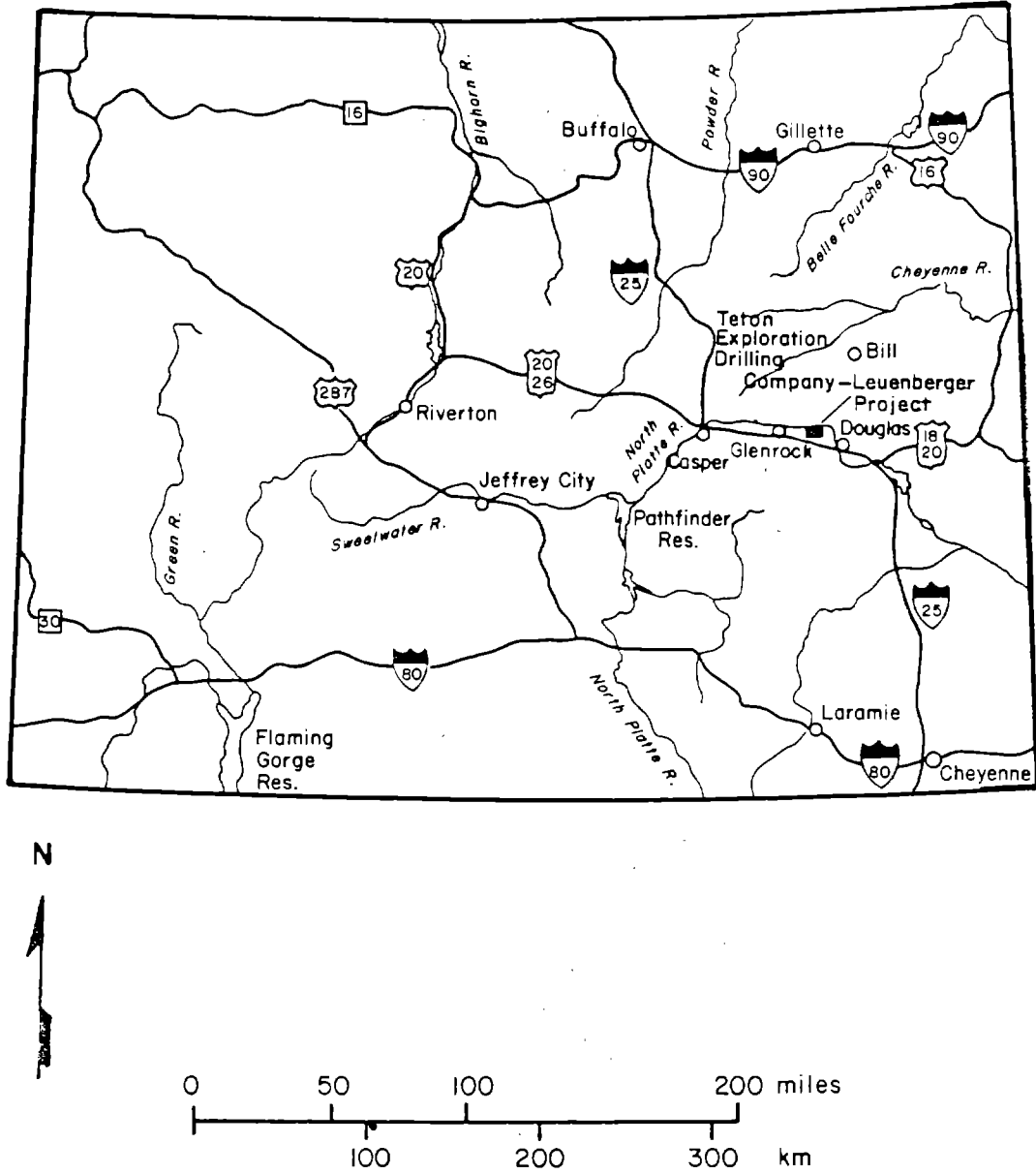
Fig. A.39. Location map of the Teton Exploration Drilling Company Leuenberger mine.
