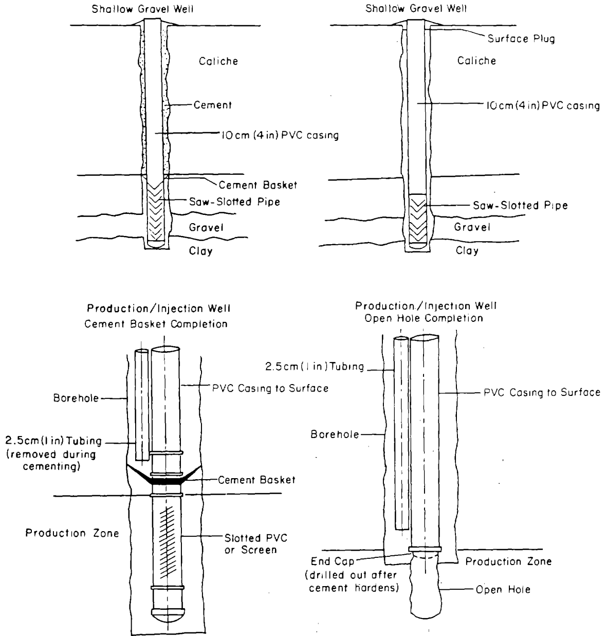
Fig. A.67. Typical well completion methods for the Brunni mine. Source: WMC, 1979a.
