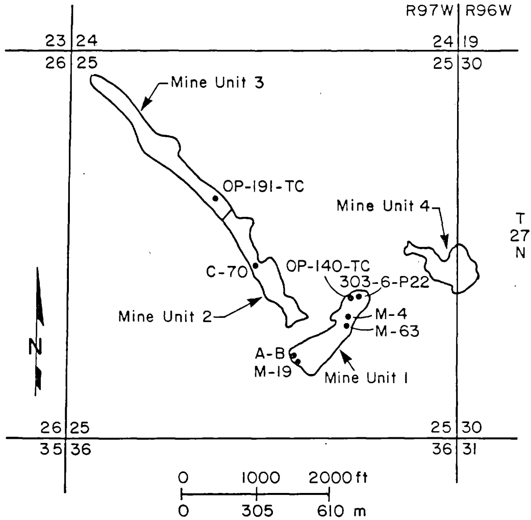
Fig. A.14. Location map of pumping/injection wells for the aquifer tests conducted at the Bison Basin mine site. Source: Modified from NRC, 1981a.
