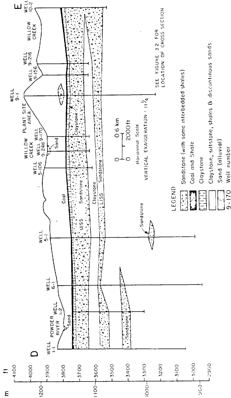
Fig. A.8. Simplified cross section through the Irigaray site. Source: NRC, 1978a.
