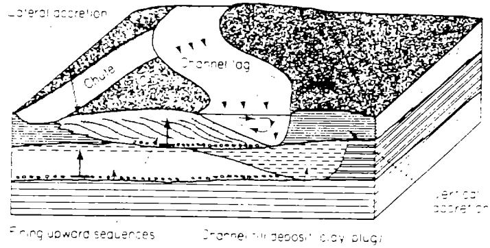
Fig. 2.5. Block diagrams showing main features of a meandering river and its floodplain. Source: Blatt et al., 1980.
