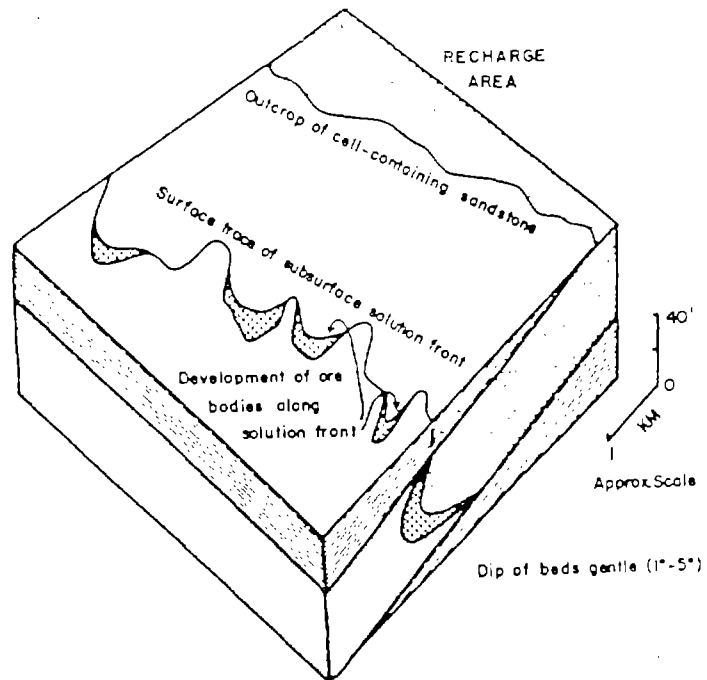
Fig. 2.2. Typical uranium roll-front deposit. Source: Campbell and Biddle, 1977.
