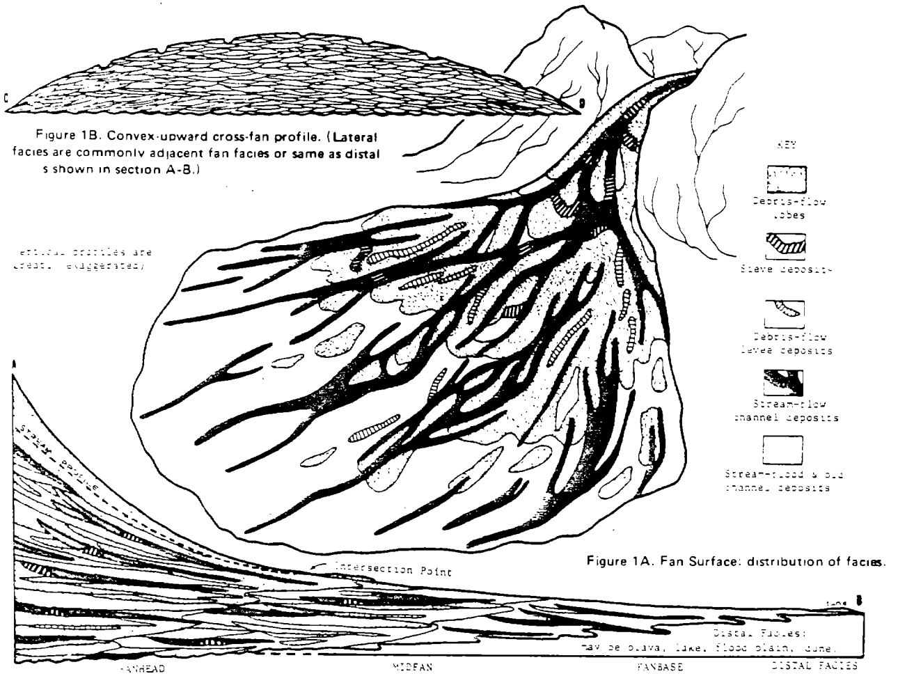
Fig. 2.7. Distribution of sediment facies and morphological profiles of an ideal alluvial fan. Source: Spearing, 1975.
